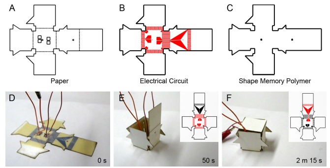
Fig. 4. Electrically activated self-folding cube. A-C) Designs of three layers that compose the electrically activated laminate: a paperboard mechanical layer (A), a copper clad polyimide electrical layer (B), and a pre-strained polystyrene shape memory polymer layer (C). D-F) Frames from self folding experiment. A power supply was used to run two amperes of current through the sub-circuits indicated in red on the insets. The time of each frame is indicated.
